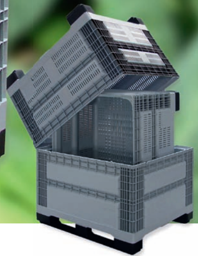
Thanks to secured counter stacking, 3 empty Paloxes can be stored in a space-saving fashion. Space savings: 33 %.
